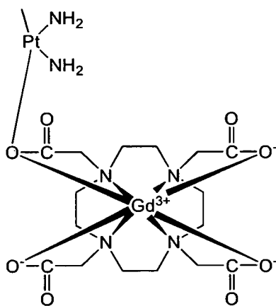
[Chemical formula 54]
