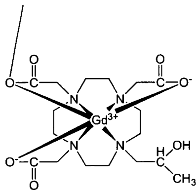
[Chemical formula 73]
