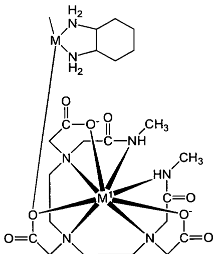
[Chemical formula 20]
