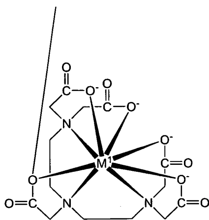
[Chemical formula 7]
