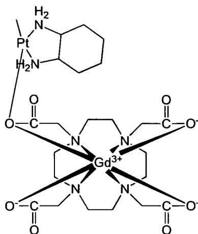
[Chemical formula 55]
