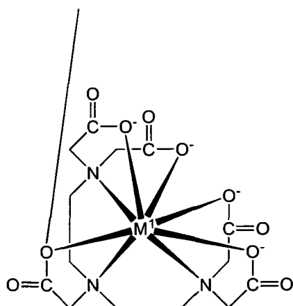
[Chemical formula 66]
