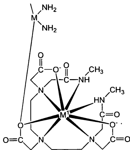
[Chemical formula 19]
