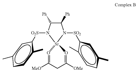
[Complex B]
