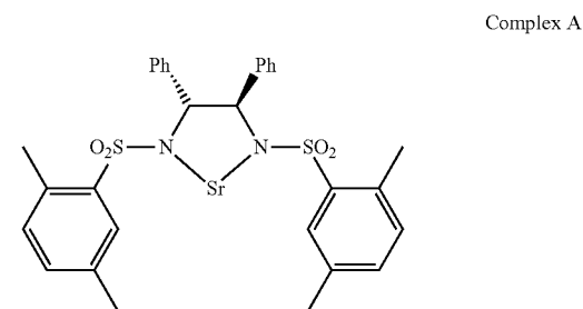
[Complex A]
