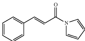
3-Phenyl-1-(1H-pyrrol-1-yl)prop-2-en-1-one
