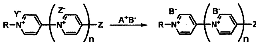
[Chemical Equation 6]
