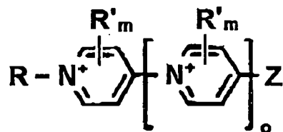
[Chemical Formula 3]
