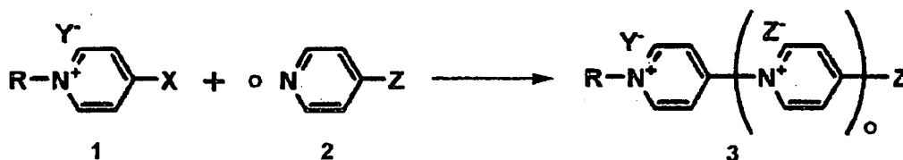
[Chemical Equation 4]
