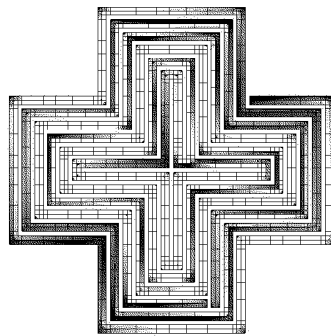
(a) 1.5GHz
