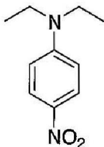
N,N-diethyl-4-nitroaniline
