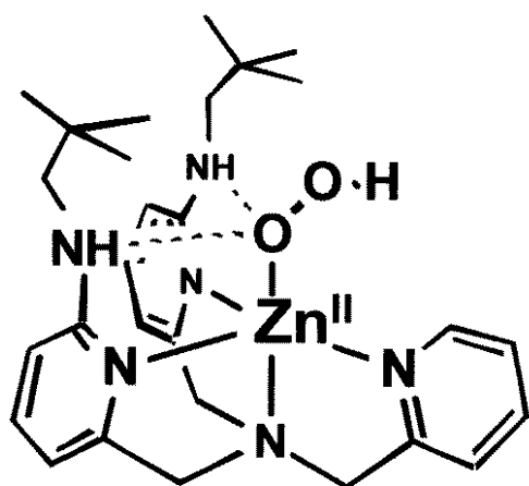
[Zn(bnpa)(OOH)] +
