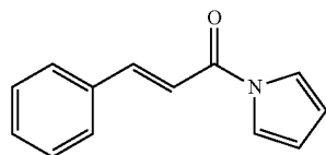
3-Phenyl-1-(1H-pyrrol-1-yl)prop-2-en-1-one
