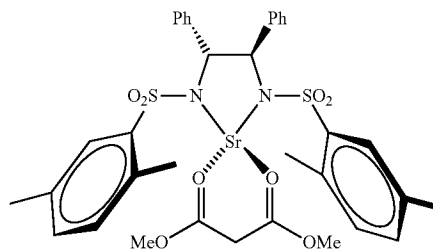
[Complex B]
