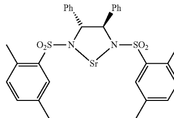
[Complex A]
