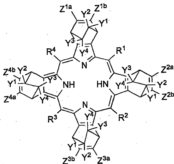
[Chemical Formula 28]
