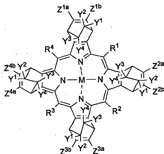
[Chemical Formula 29]
