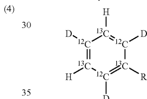
Phenylalanine
