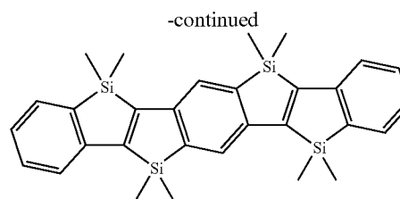
Silicon Cross-Linked Stillbene and a Derivative Thereof
