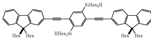
Scheme 7
