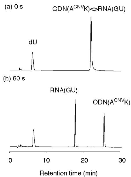
Figure 12. HPLC analysis.
