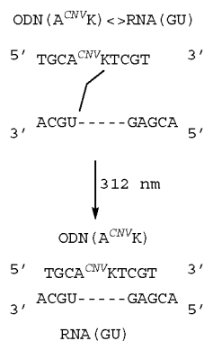
Scheme 7
