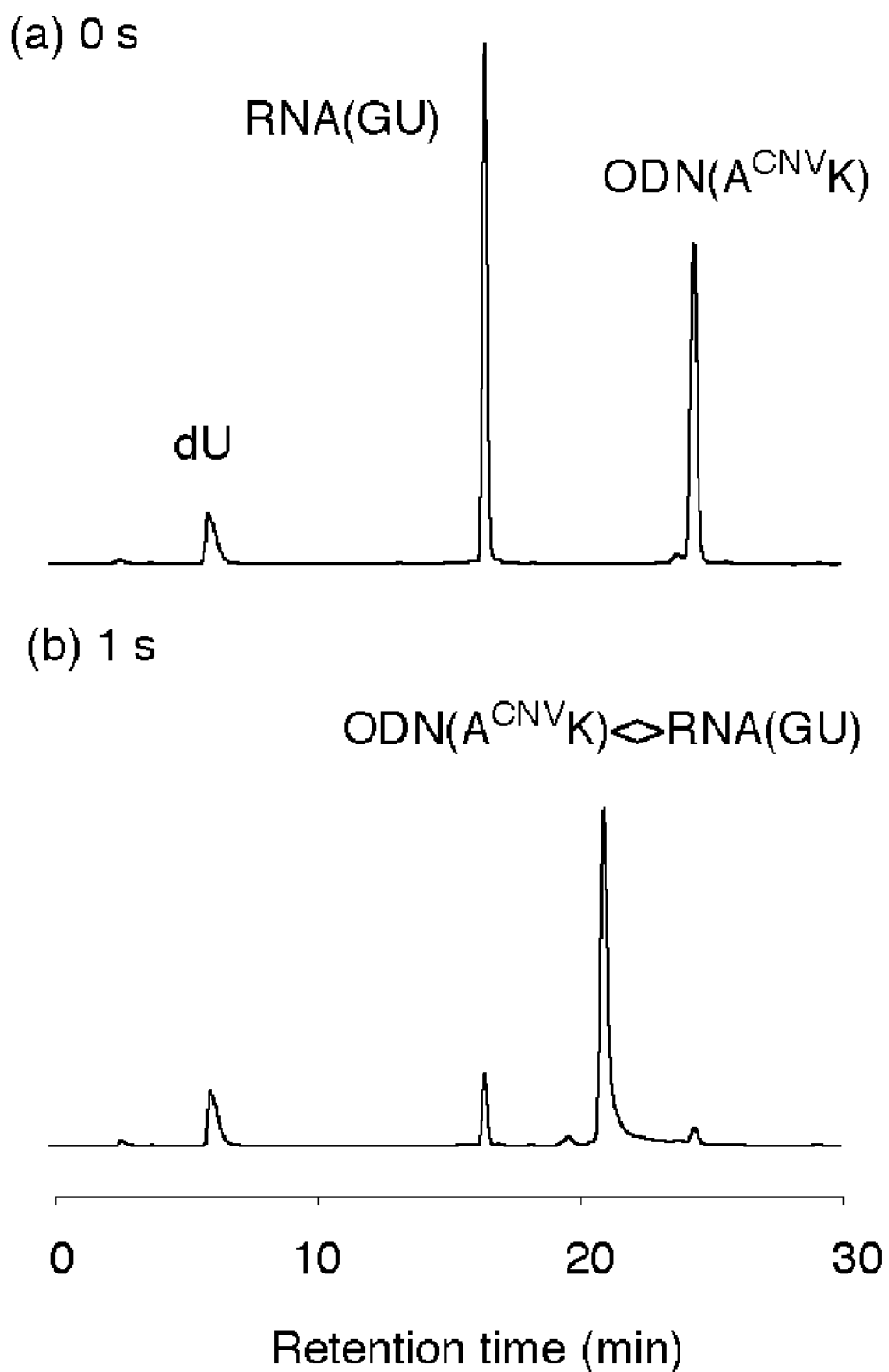
Figure 10. HPLC analysis.
