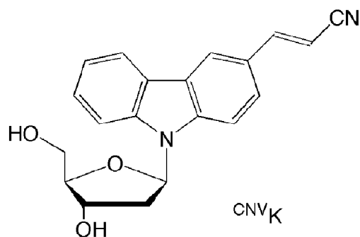
Figure 1. Structure of 3-cyanovinylcarbazole-1'-β-deoxyribose.
