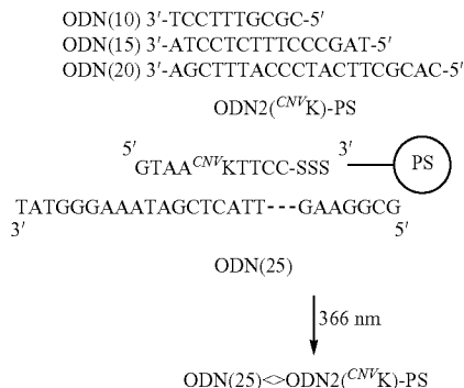
Scheme 5.
