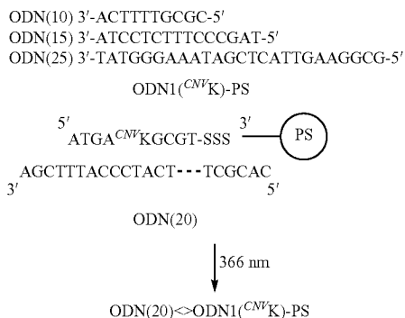
Scheme 4.
