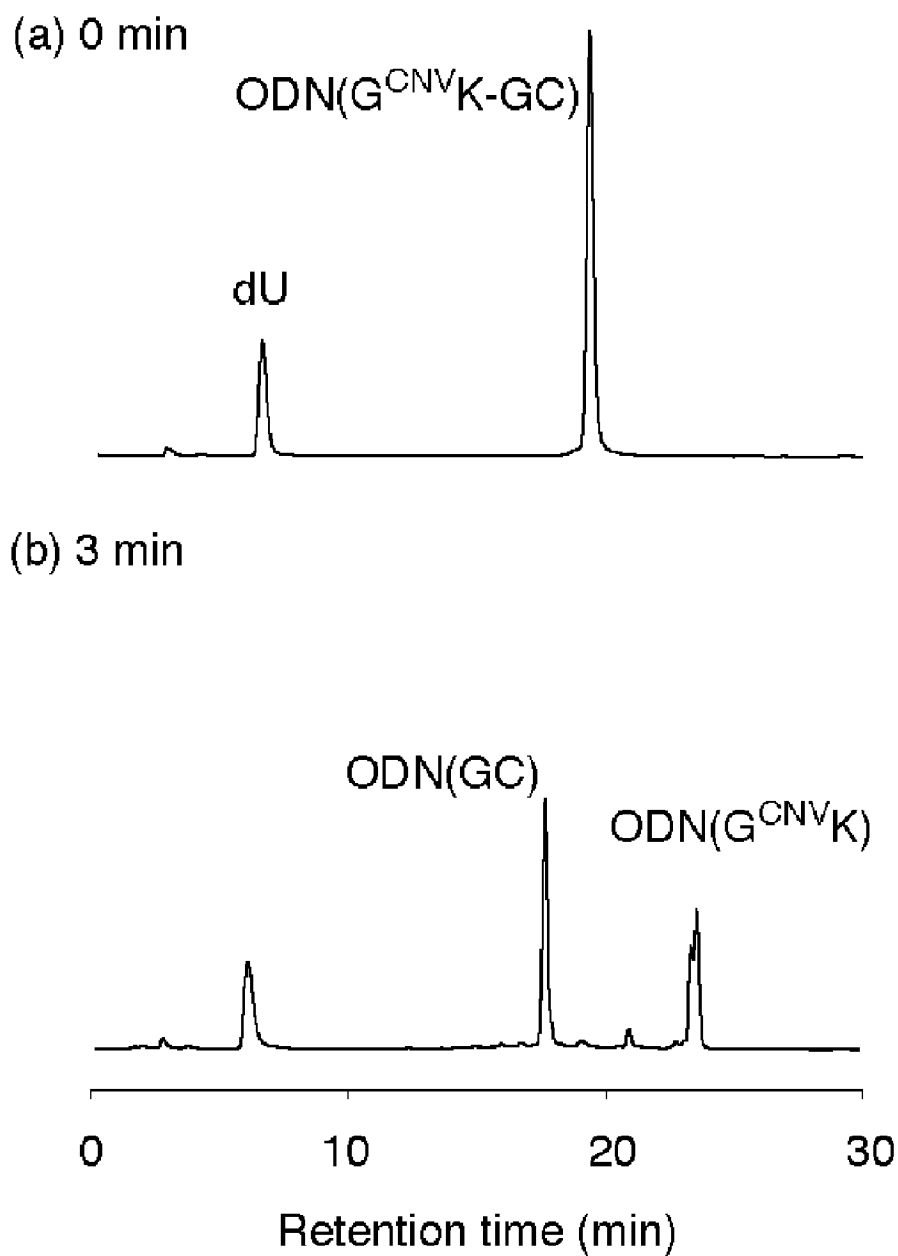
Figure 3. HPLC analysis.
