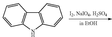
Scheme 9
