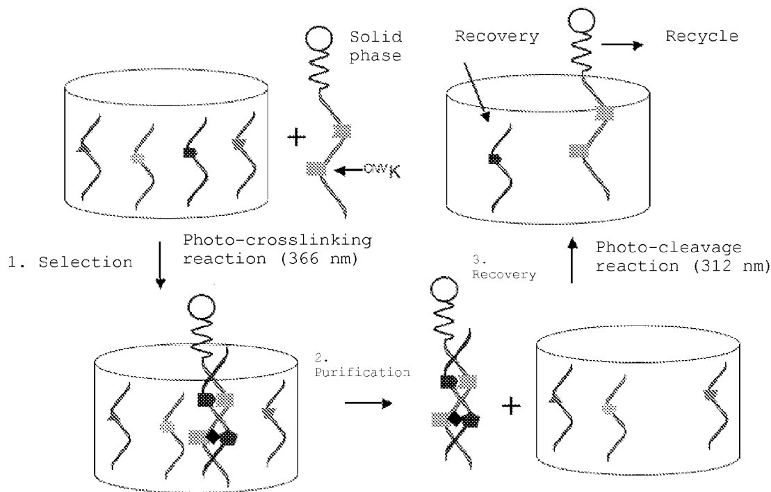
Strategy for the sequence specific purification of DNA.
