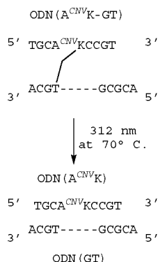
Scheme 3.
