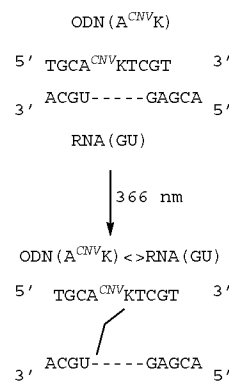
Scheme 6.
