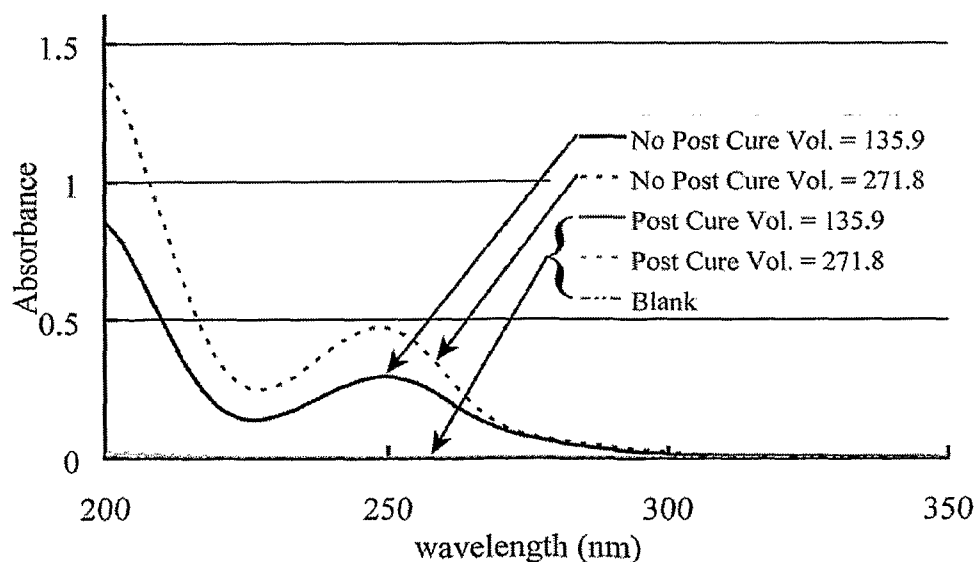
Ultraviolet absorption spectrum
