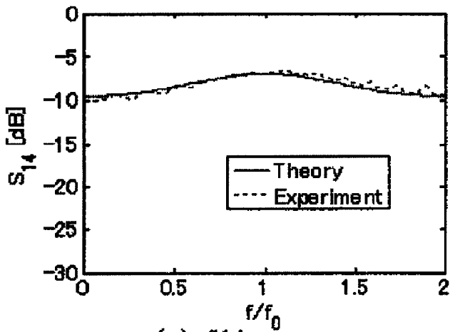
(c) S_{14}
