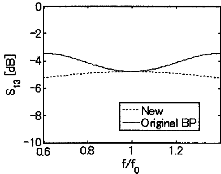
(b) S_{13}
