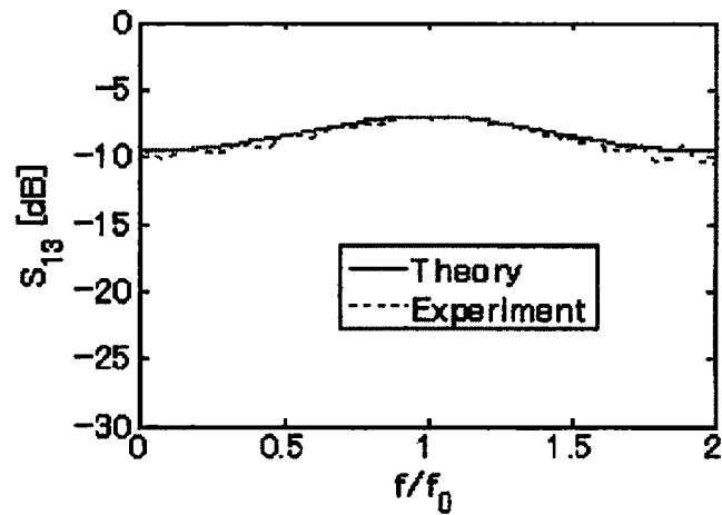
(b) S_{13}
