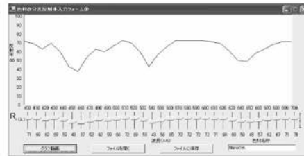
NanoTek Powderの分光反射率
