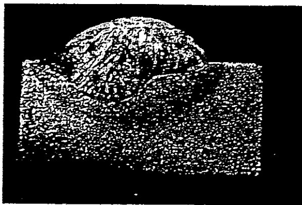
(c) 100%CO 2
