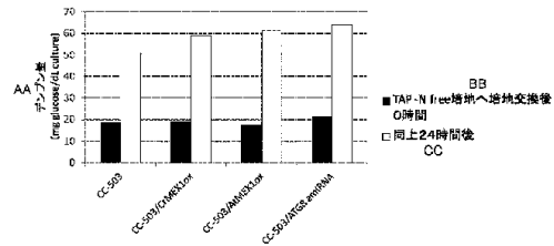
AA... AMOUNT OF STARCH (mg glucose/dL culture) BB... 0 HOURS AFTER CHANGING MEDIUM TO TAP-N free MEDIUM CC... 24 HOURS AFTER CHANGING MEDIUM TO TAP-N free MEDIUM
