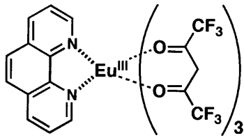
\text{Eu}(\text{hfa})_3(\text{phen})
