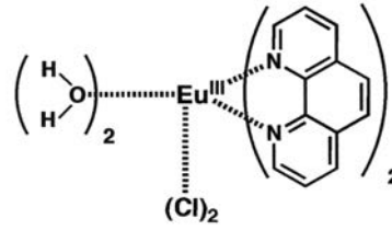
\text{Eu}(\text{phen})_2\text{Cl}_2(\text{H}_2\text{O})_2
