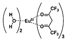
\text{Eu}(\text{hfa})_3(\text{H}_2\text{O})_2
