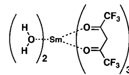
Sm ( h f a ) 3 ( H 2 O ) 2
