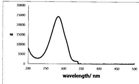
Eu ( h f a ) 3 ( p h e n )
