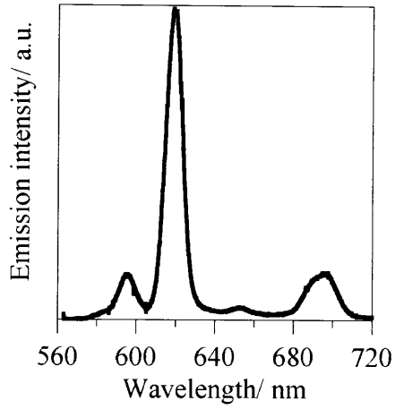
\text{Eu}(\text{hfa})_3(\text{phen})
