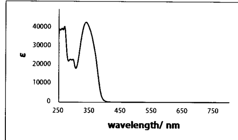
\text{Eu}(\text{ntfa})_3(\text{H}_2\text{O})_2
