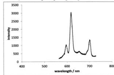
\text{Eu}(\text{phen})_2\text{Cl}_2(\text{H}_2\text{O})_2
