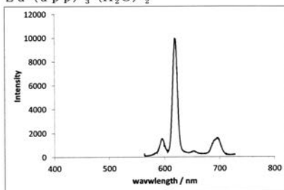
\text{Eu}(\text{dpp})_3(\text{H}_2\text{O})_2
