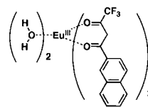
\text{Eu}(\text{ntfa})_3(\text{H}_2\text{O})_2
