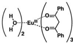
\text{Eu}(\text{dpp})_3(\text{H}_2\text{O})_2
