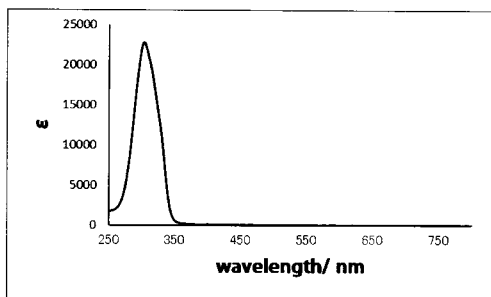
\text{Eu}(\text{hfa})_3(\text{H}_2\text{O})_2
